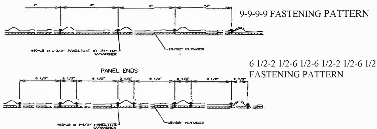
TEST A & B FASTENER PATTERN
